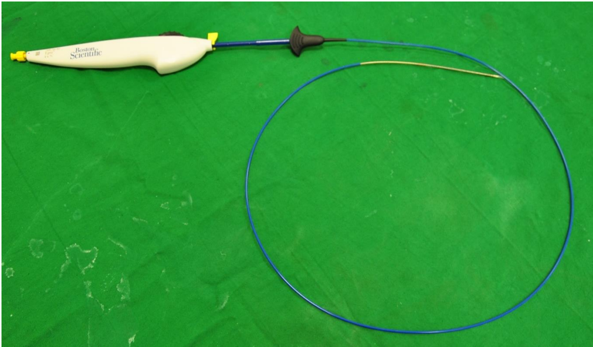
(7) Over the wire Self expanding Nitinol Stent with Delivery System
