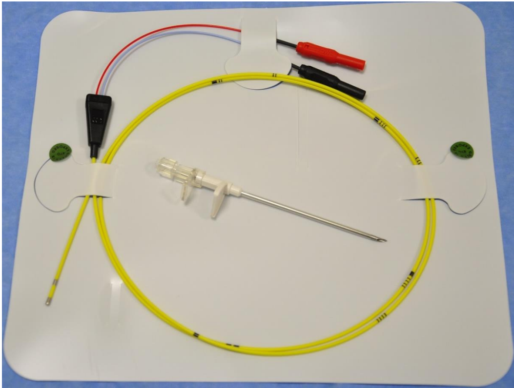
(11) VascoStim Intracardiac lead for temporary pacing and electro physiology (Arrow)
